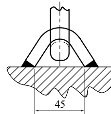
Welding Recommendation
